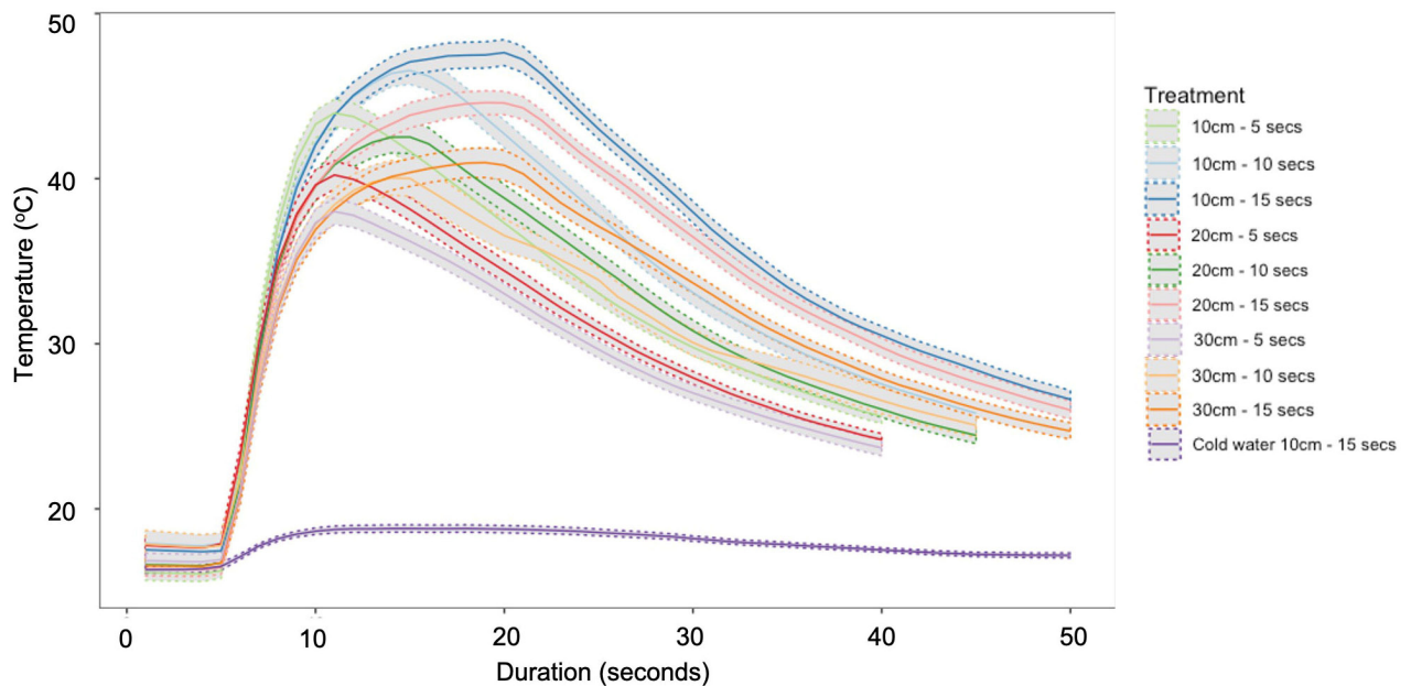
Figure 2. Average temperature of hot water spray treatment applied to Dreissena polymorpha , Dikerogammarus villosus and Crassula helmsii from three distances (10, 20, 30 cm) and for three durations (5, 10, 15 seconds) and control cold water treatment (from 10 cm for 15 seconds). Grey shading shows standard error of average (n = 36).
