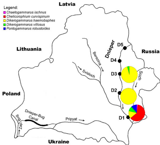
Figure 1. Belarusian section of the Dnieper River and its main tributaries (modified from Karatayev et al. 2000). D1-D5 are stations sampled in this study. Pie-charts characterise composition of alien gammarid communities as % total number of individuals sampled.
