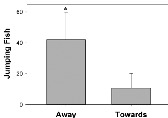
Figure 9. Average number of fish that jumped “away” from versus “towards” the boat. Averages were calculated based on pooling the total number of jumping fish in response to each outboard motor type at one of the four speeds (100 hp @ 16 km/hr, 100 hp @ 24 km/hr, 100 hp @ 32 km/hr, and 100 hp @ 40 km/hr, 150 hp @ 16 km/hr, 150 hp @ 24 km/hr, 150 hp @ 32 km/hr, and 150 hp @ 40 km/hr), * indicates significantly different groups (t-test P < 0.001 ). Error bars represent \pm SE.
