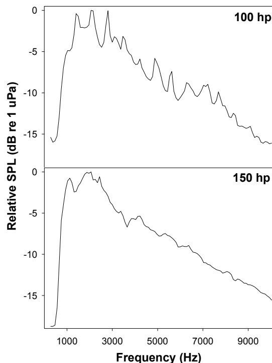
Figure 2. The power spectrum in relative dB of the 100 and 150 hp outboard motors is plotted versus frequency (Hz).
