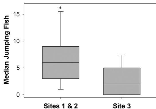
Figure 3. Median jumping silver carp in pooled Sites 1 and 2 versus Site 3. Each box represents the 25 th (bottom of box) and 75 th (top of box) quartiles with the median marked by the line within the box. Whiskers (error bars) above and below the box indicate the 10 th and 90 th percentiles. * indicates significantly different group (Mann-Whitney P < 0.001 ).
