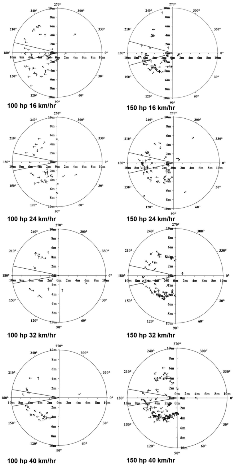
Figure 5. Polar plots for all eight treatments. Each arrow represents one fish and marks the estimated distance from and jump initiation angle in relation to the boat and its direction of movement (0°). To assess the jumping vector, each fish was categorized in one of eight arcs (0°–45°, 46°–90°, 91°–115°, 116°–135°, 136°–180°, 181°–270°, 271°–315°, and 316°–360°) and plotted with a corresponding arrow. The arrows point in the direction of each fish’s trajectory (jumping vector). The solid lines represent the boat’s wake.
