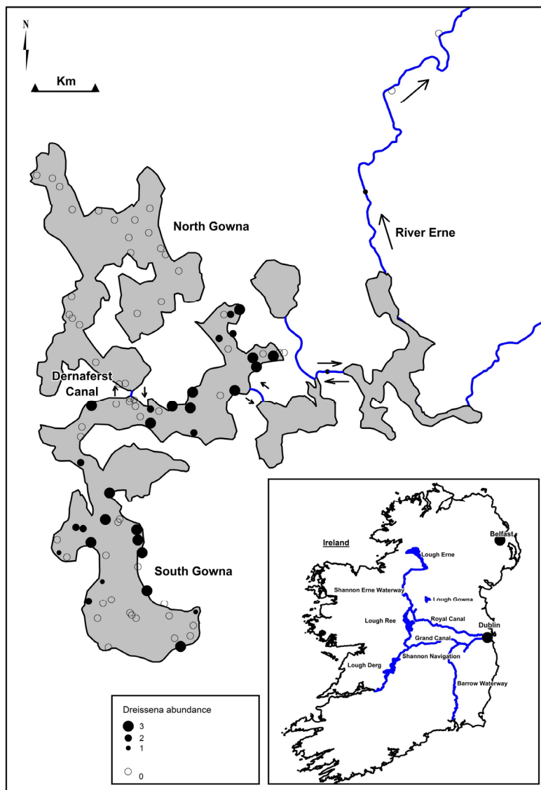
Figure 1. The inland waterways of Ireland and position of Lough Gowna. Lough Gowna and Erne River showing distribution of stations and assessment units North Gowna (NG), South Gowna (SG) and the Erne River (ER). Arrows indicate water flow directions. Mussel abundance 0 absent, 1 low, 2 moderate and 3 abundant.
